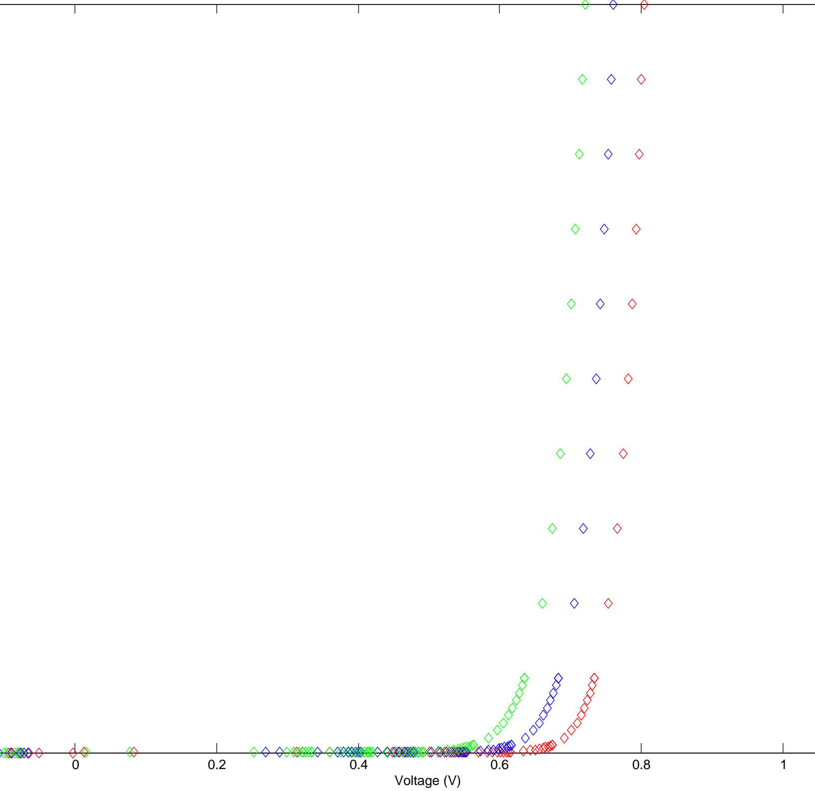
Diode Band Gap: V vs I Curves at Different Temperatures
