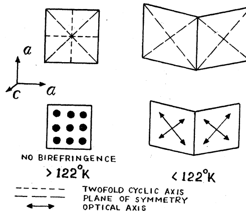
FIG. 2. Symmetry element and double refraction of \text{KH}_2\text{PO}_4 .
