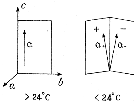
FIG. 1. Deviation of the optical axis a caused by spontaneous deformation in rochelle salt.
