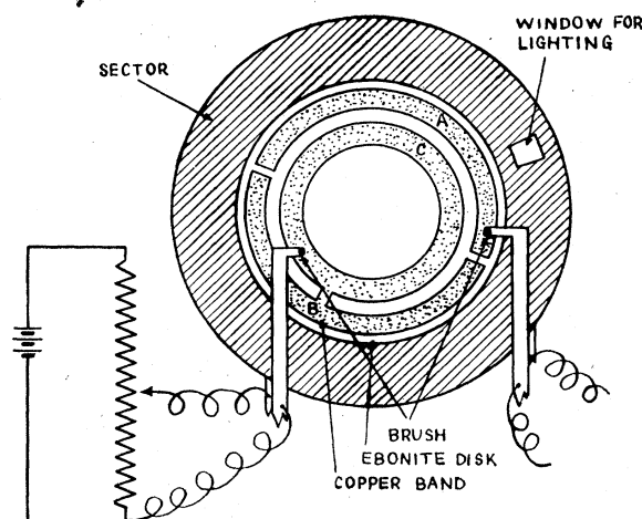
FIG. 12. Apparatus to study the motion of the wall for square wave voltage.
