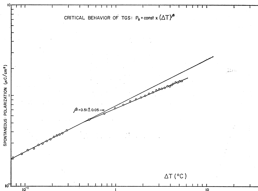
FIG. 1. Log-log plot of spontaneous polarization versus temperature for ferroelectric triglycine sulfate in the vicinity of the critical temperature.
