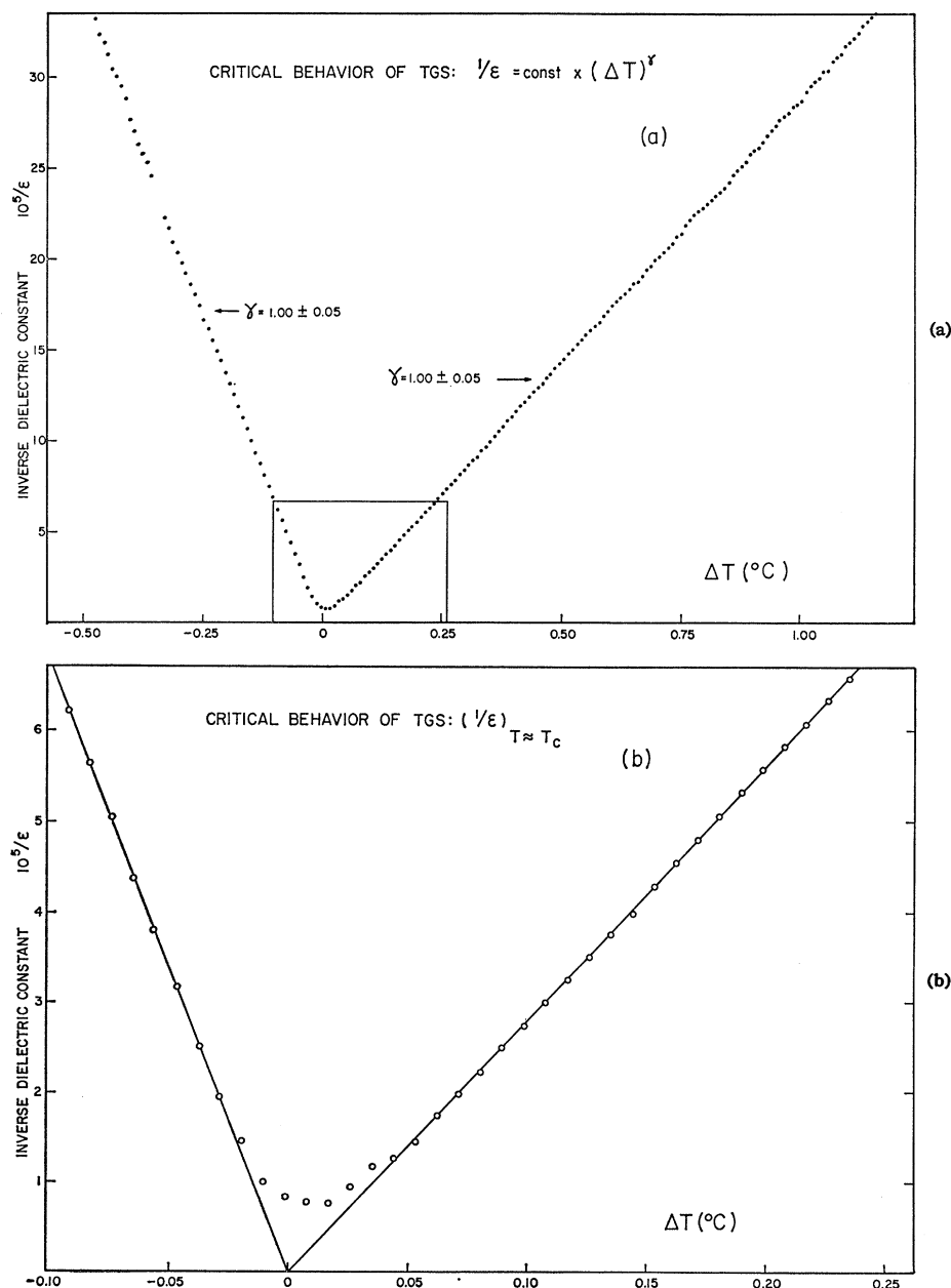
FIG. 2. (a) Plot of the inverse dielectric constant versus temperature ( T_c = 49.42 \pm 0.05^\circ\text{C} ). (b) Detail of the same plot as in (a) (portion squared) in larger scale, showing behavior in the immediate vicinity of T_c .
