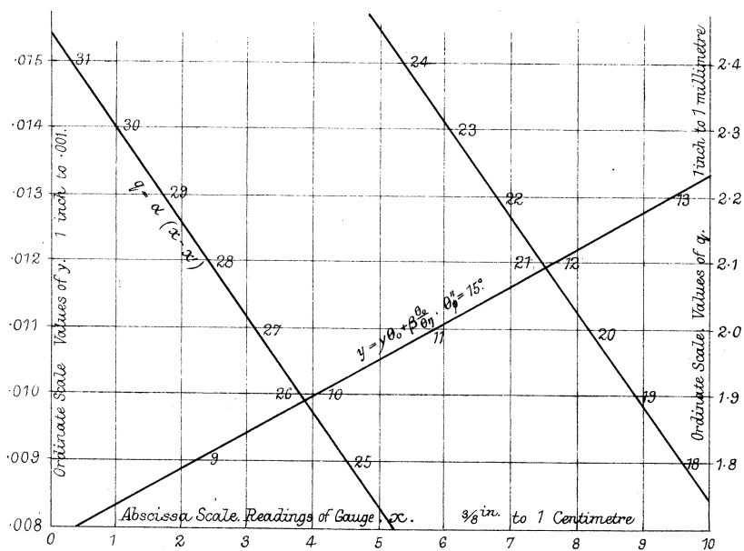
CORRECTION DIAGRAM Air Thermometer N° 2.
